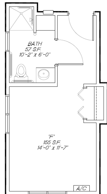
STYLE F - 315 SQ. FT.
