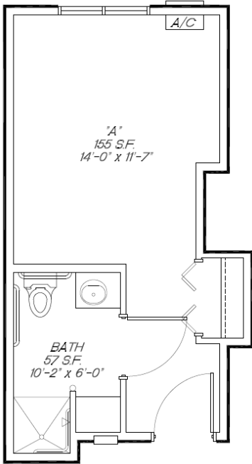
STYLE A - 300 SQ. FT.
