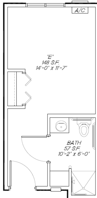
STYLE E - 305 SQ. FT.
